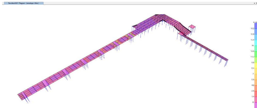
Gambar 4.5 Contour M11 Slab
