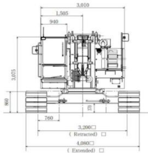
Gambar 3.3 Dimensi Crawler Crane Tampak Depan
