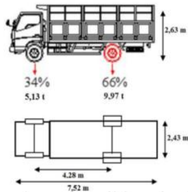
Gambar 3.1 Dimensi Truck
