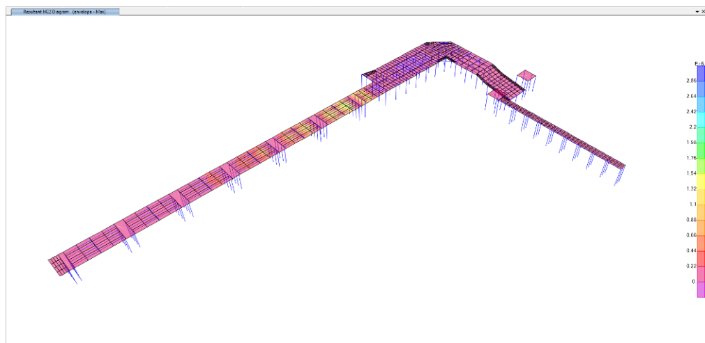
Gambar 4.6 Contour M22 Slab
