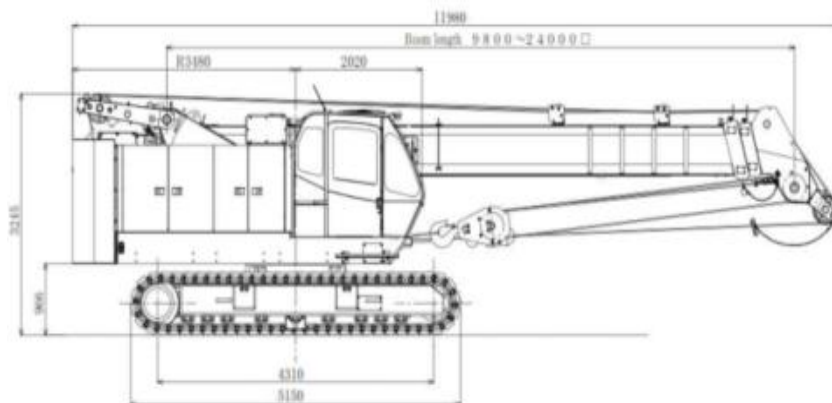
Gambar 3.2 Dimensi Crawler Crane Tampak Samping
