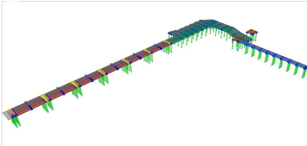
Gambar 4.2 3D View Struktur (Extrude)
