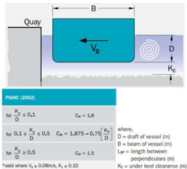
Gambar 3.5 Perhitungan koefisien CM
