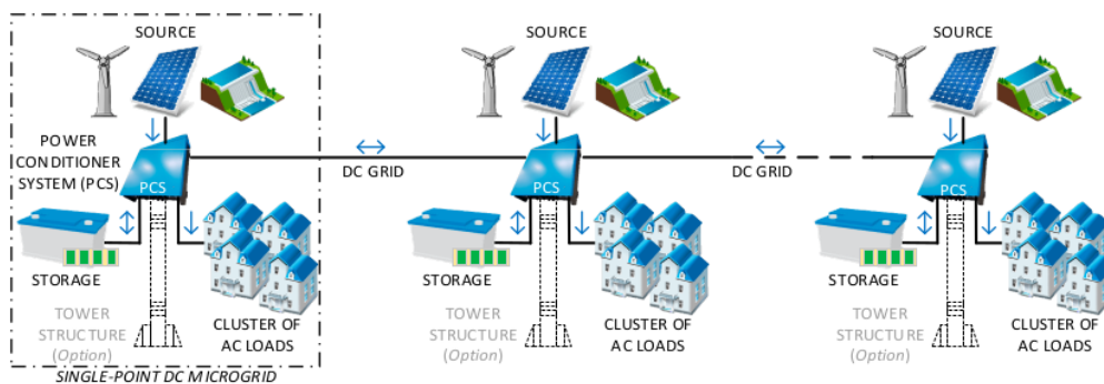
Figure 1. The proposed DC microgrid system.
