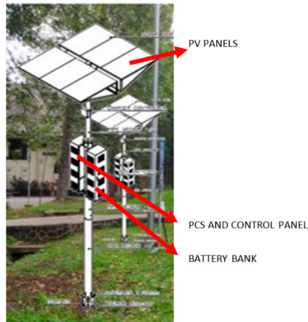
Figure 6. Solar tower: An implementation of PCS.
