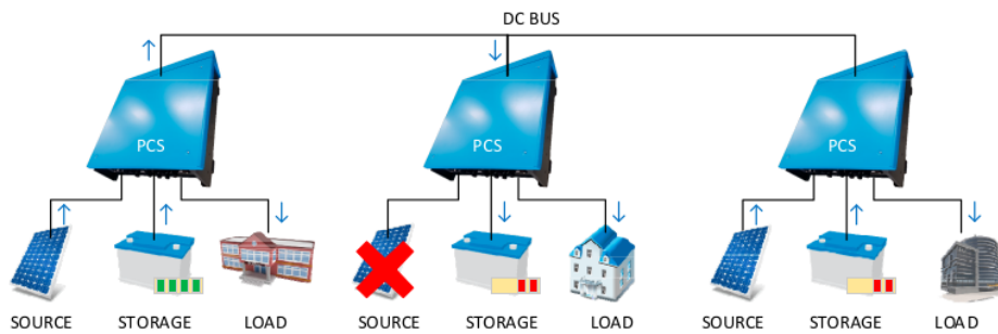
Figure 5. Power flow in multi-point DC microgrid system.
