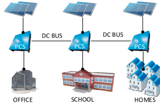
Figure 4. Multi-point DC microgrid configuration.
