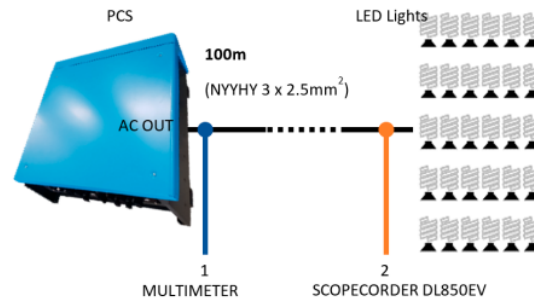
Figure 7. PCS field evaluation with distant loads.
