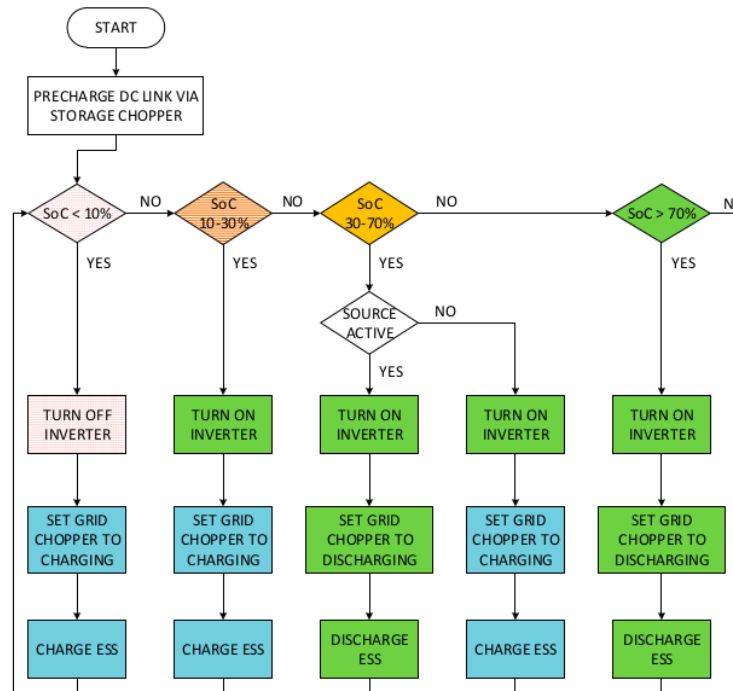
Figure 3. Flowchart of the PCS management unit.
