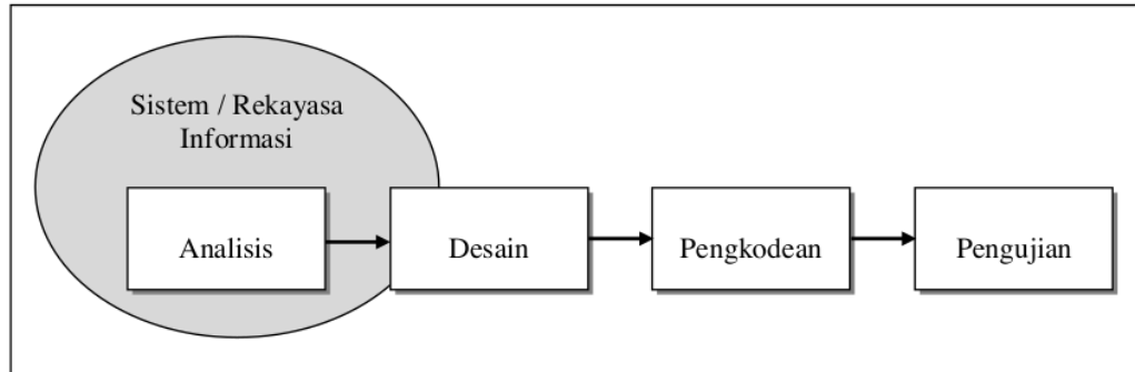
Gambar 1. Metode Waterfall [7]
