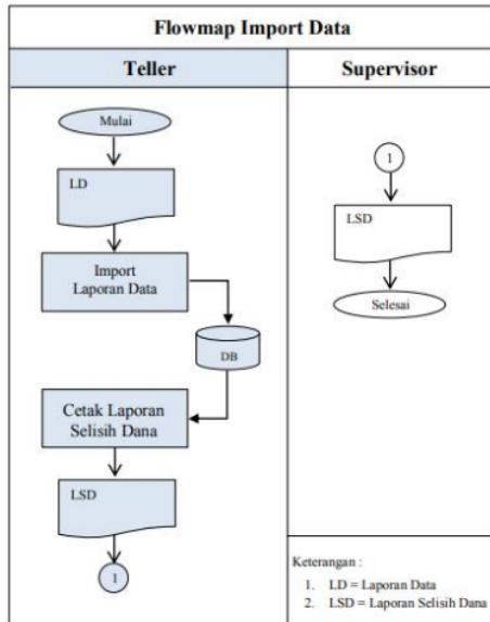
Gambar 2. Flowmap Import Data Usulan
