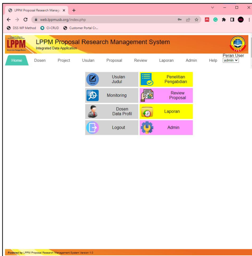
Gambar 3. Halaman Home
