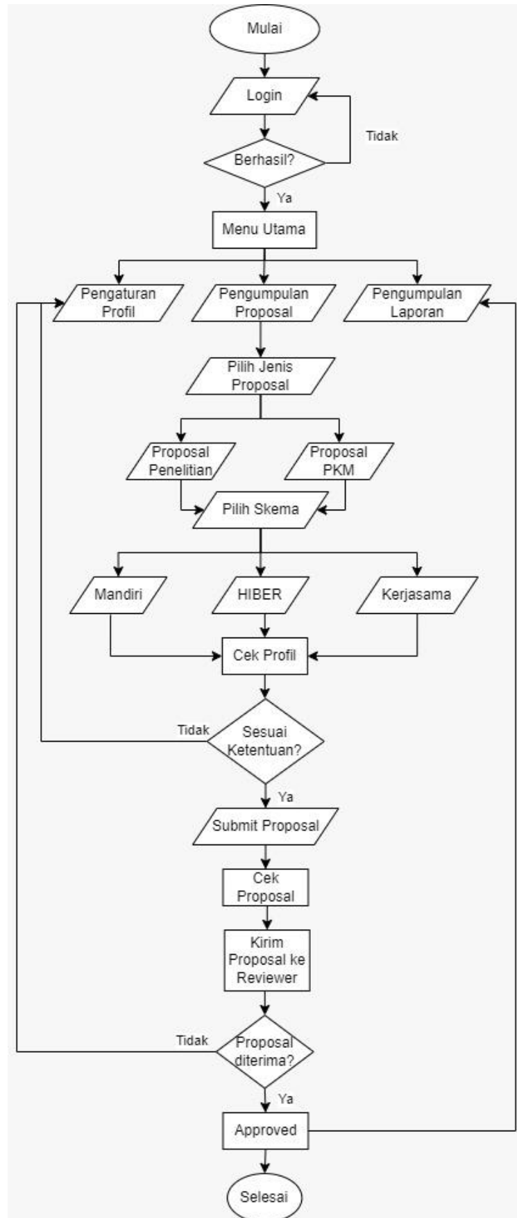
Gambar 1. Flowchart Sistem
