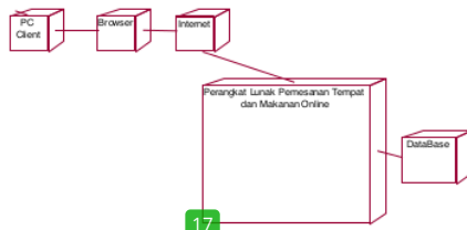
Gambar 3. Deployment Diagram
