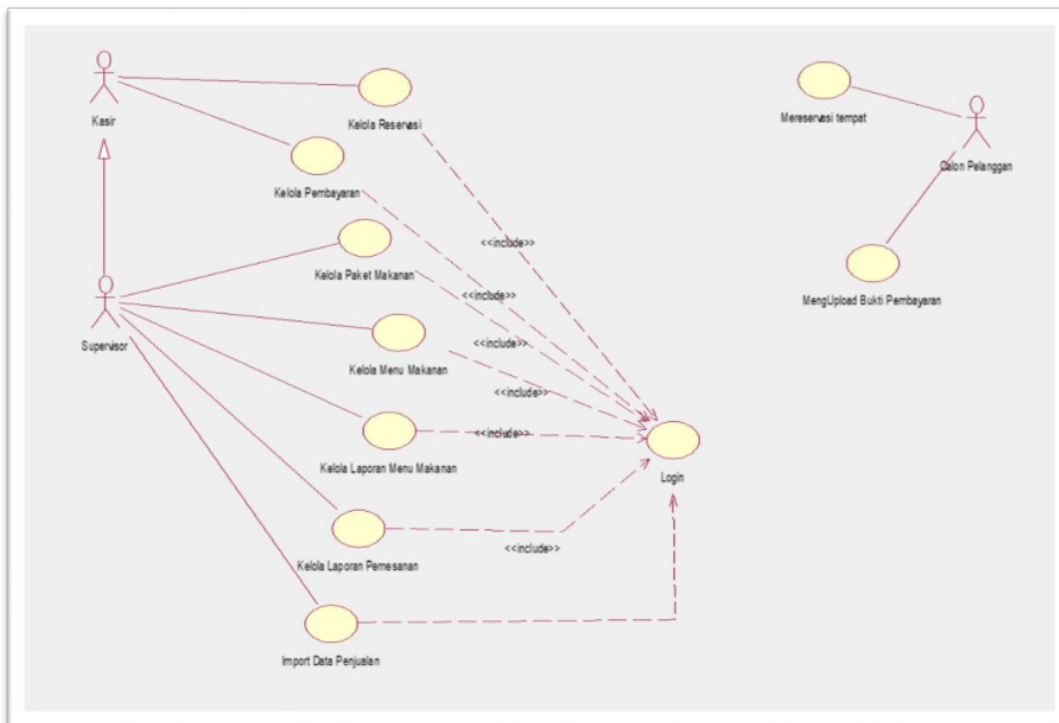
Gambar 1. Usecase Diagram
