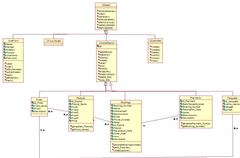
Gambar 2. Class Diagram
